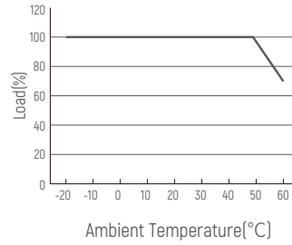
Derating Curve
