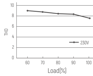
THD vs Load
