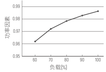
PF vs 负载
